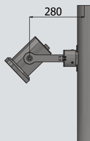
Spot + Pole fitting.
